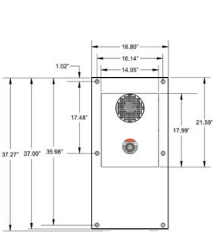
Bottom View
