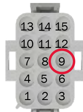
J8 Wire Insertion View Shown
